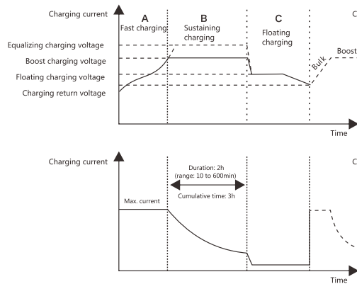
Fig. 1-5 SLD Battery charging stages diagram
