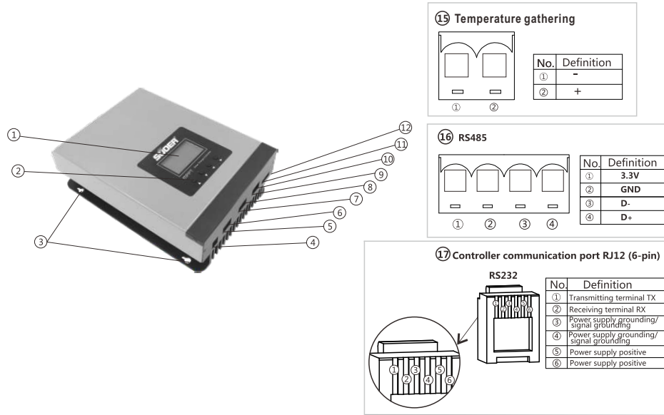
Fig. 1-1 Product appearance and interfaces
