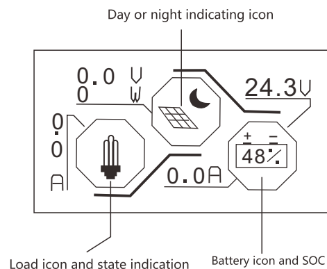
Definitions of "main menu" icons
