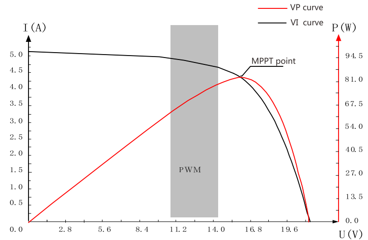
Fig. 1-2 Solar panel output characteristic curve
