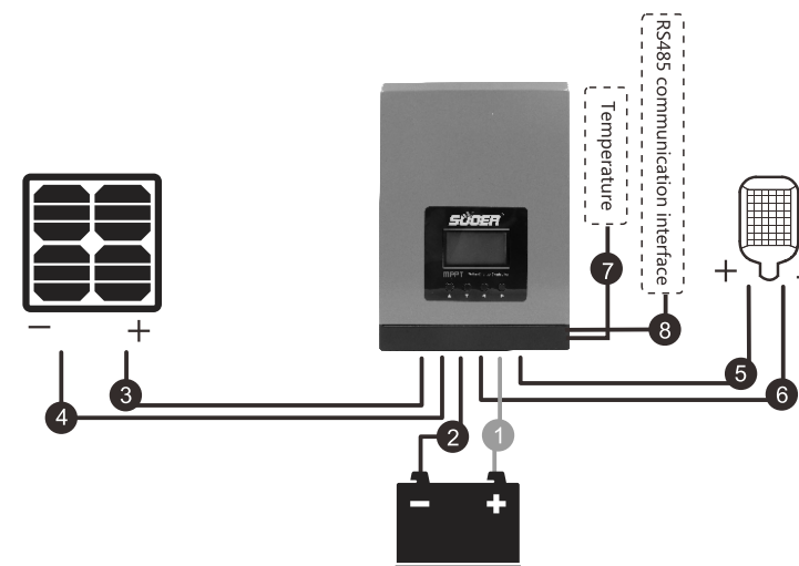
Fig. 2.3 Wiring sequence
